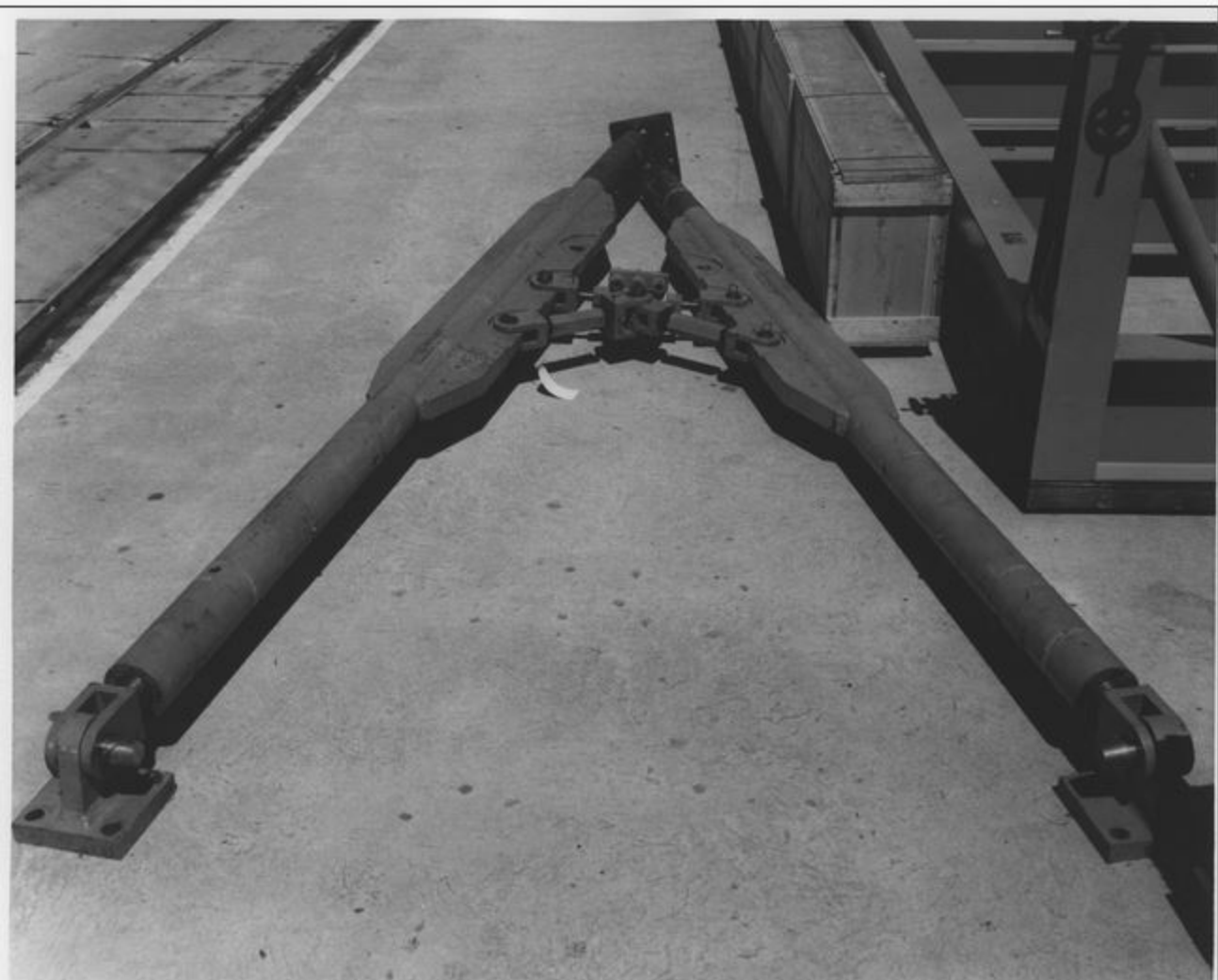
SSBN-600 "A" FRAME FOR BRIDGE CRANE (LOWER PADS FIT HULL PADS UNDERWATER)
