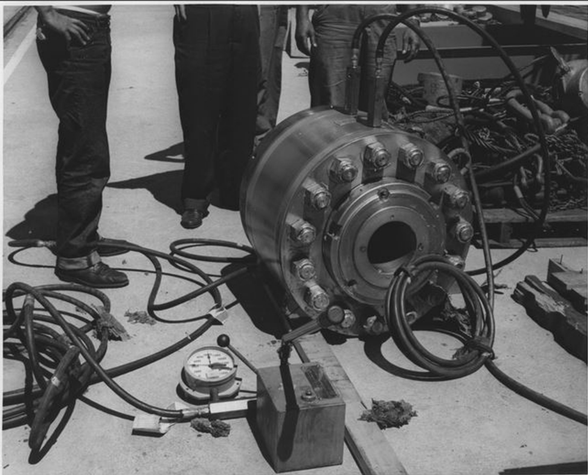
SSBN-600 HYDRAULIC JACK UNIT FOR REMOVING & INSTALLING PROPELLER
