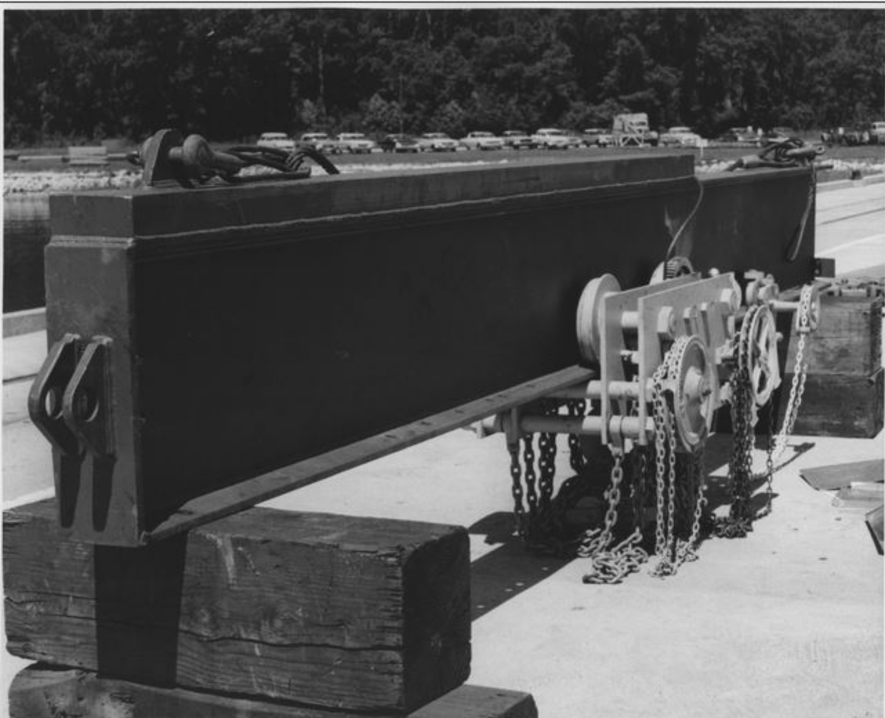
SSBN-600 BRIDGE CRANE ASS'Y FOR WATER BORNE PROPELLER CHANGE
