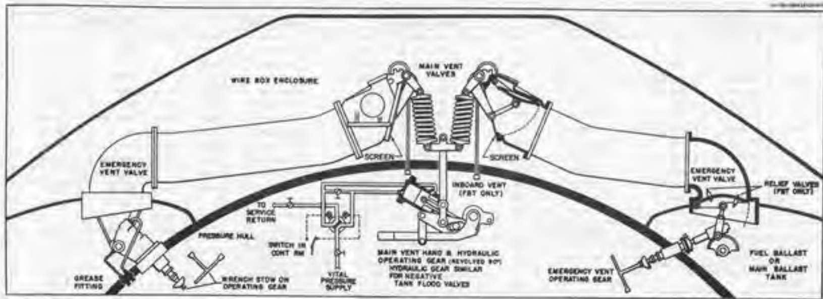
TYPICAL MAIN AND EMERGENCY VENT ARRANGEMENT
