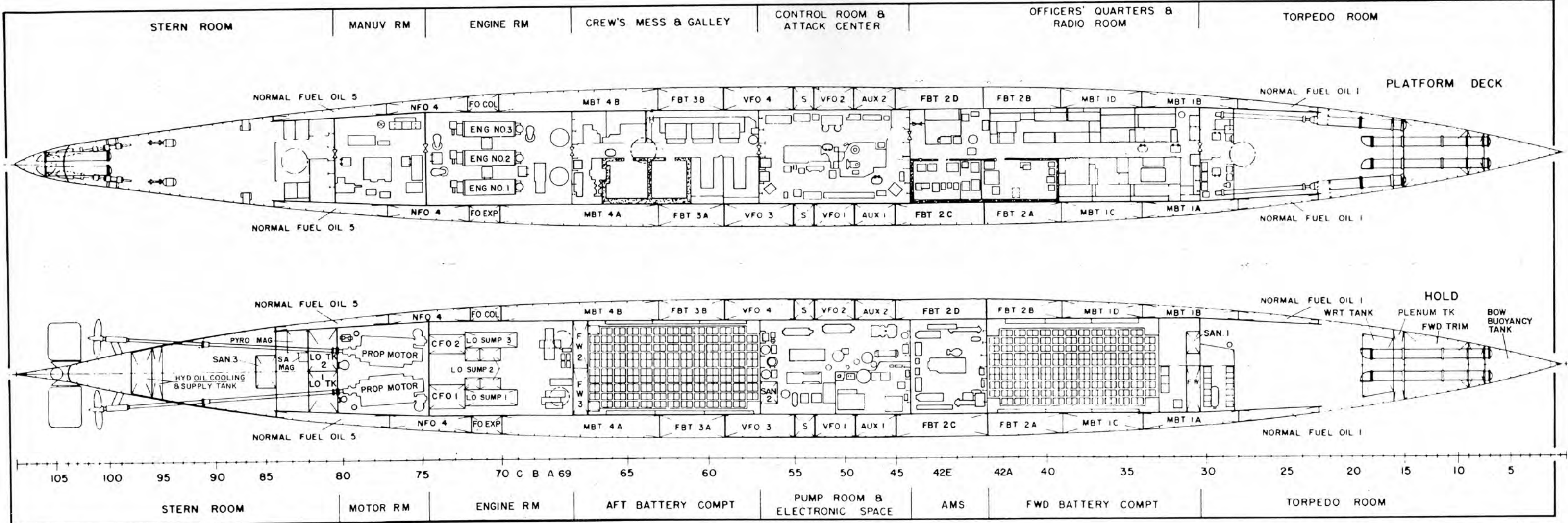
PLATFORM DECK & HOLD
