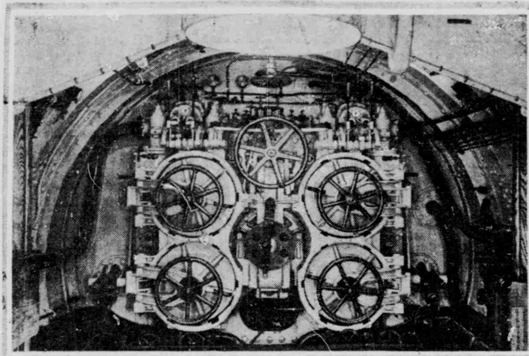
TORPEDO TUBES OF A SUBMARINE This remarkable photograph shows the four torpedo tubes of the Spanish submarine Isaac Peral, built by the submarine Boat corporation and now undergoing trials at Provincetown, Mass. The Isaac Peral is said by experts to be almost identical in a mechanical sense to the German U-boats Deutschland and U-53. It is as large as those under-sea boats and capable of performing or accomplishing anything that they have done.
