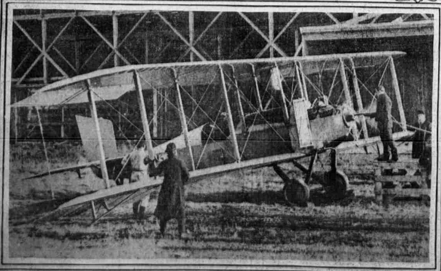
Photo by International Film Service. "STEEL BATTLEPLANE" WHICH MAY REVOLUTIONIZE AIR FIGHTING This new Sturtevant plane, now being considered by the United States Army, is twice the size of the ordinary machine and carries mountings for two gun turrets. It is built of lighter-than-wood vanadium steel and has 140-horsepower motors. It is of heavy build, so as to withstand shocks.
