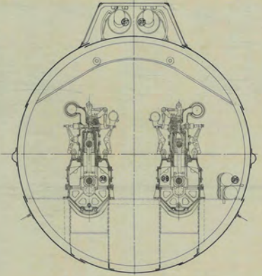
SECTION AT FRAME 32 LOOKING AFT SCALE 1/2" = 1 FT
