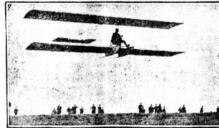
TESTING MOTORLESS GLIDER. A. H. G. Fokker, famous Dutch airplane designer, photographed while making an experimental flight on the South Downs, England. Mr. Fokker, shown in picture on the right, seated in his glider, plans to enter it in a coming competition, which carries an award of £1000
