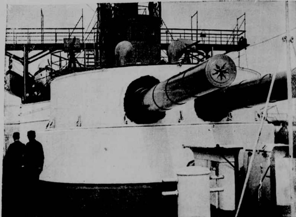
FORWARD TURRET OF THE MONITOR PURITAN.
