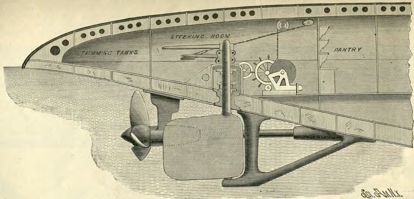
RAM "KATAHDIN"—PROPELLER AND STEERING APPARATUS.
