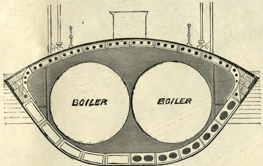
RAM "KATAHDIN"—CROSS SECTION AMIDSHIPS.
