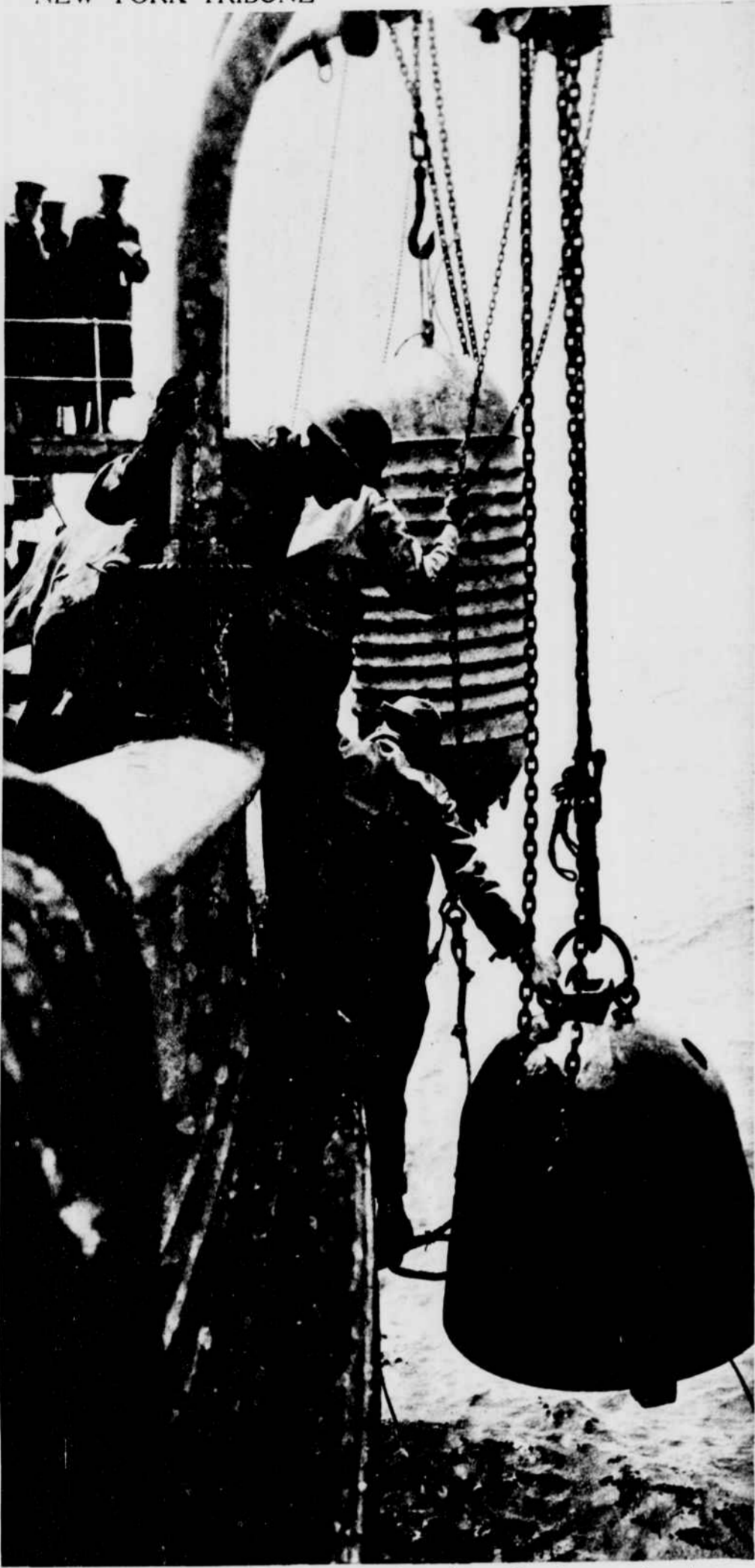
Automatic anchor swung outboard, ready to drop from a mine planter. This anchor automatically checks the outrunning mine cable at the proper depth. Photo by Bronck Breit.
