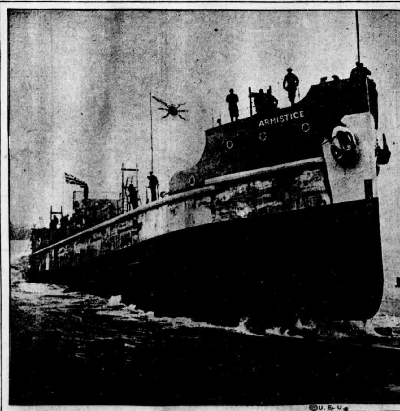
THIS IS THE LATEST addition to the fleet of British sea-going concrete vessels. The ship's name, Armistice, is new and quite up to date.
