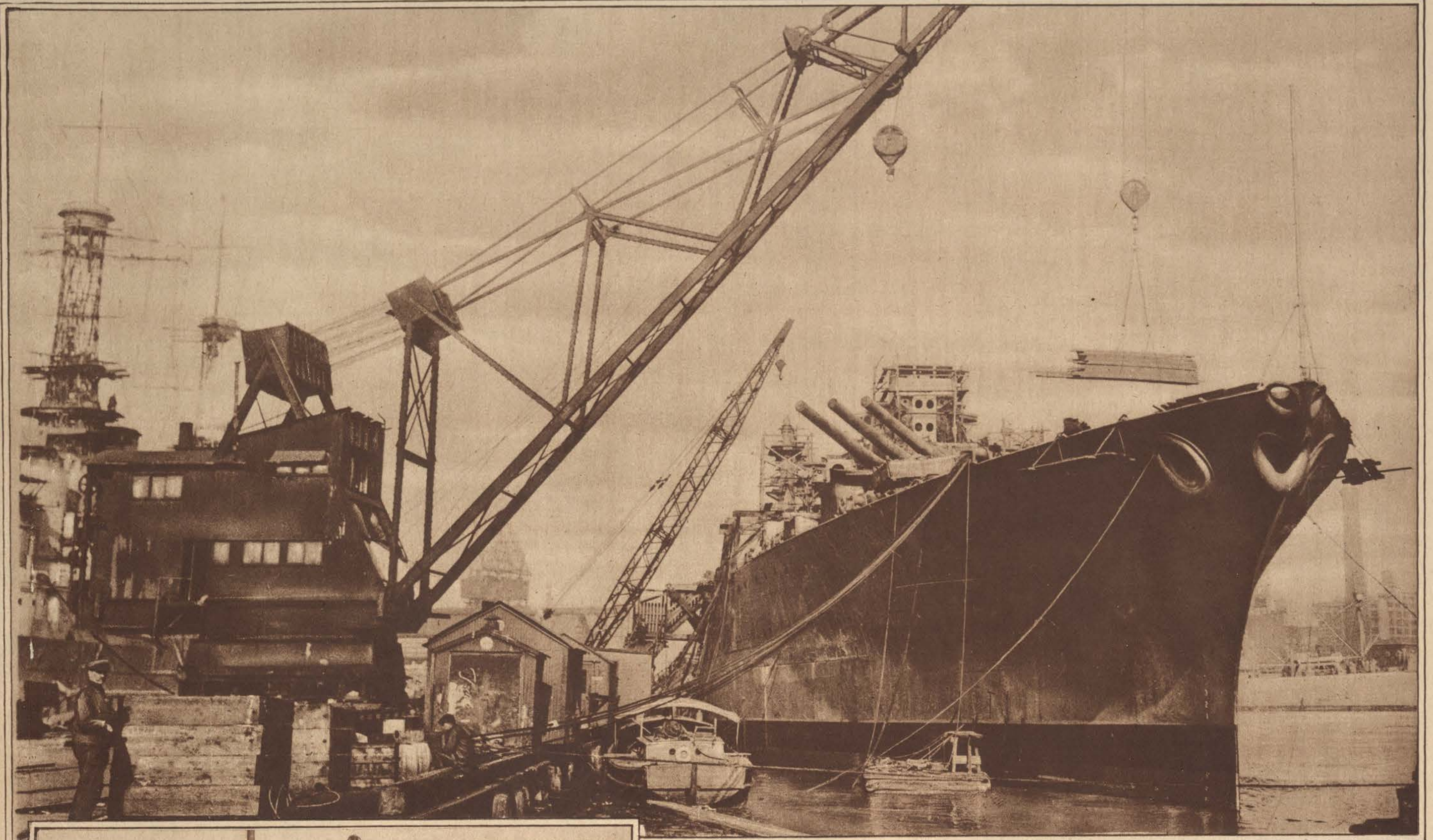
THE U. S. SUPERDREADNOUGHT TENNESSEE, LARGEST BATTLE UNIT OF THE SEA SO FAR DESIGNED FOR ANY NAVY IN THE WORLD, NOW APPROACHING COMPLETION IN THE BROOKLYN NAVY YARD. The Tennessee, Launched Last April, Is 624 Feet Long, Is an Oil Burner With Electric Drive, and Will Develop a Sustained Speed of 21 Knots an Hour. She Will Go Into Commission About Feb. 15 Next. (© Underwood & Underwood.)
