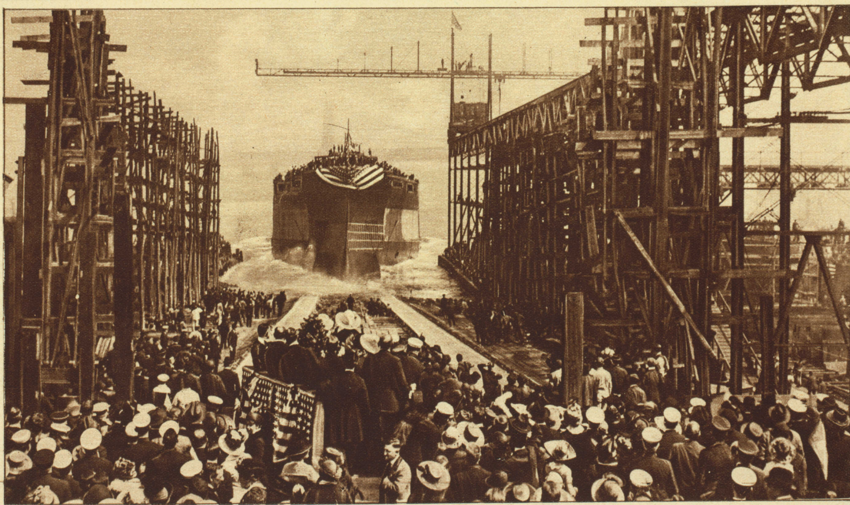
THE AMERICAN DREADNOUGHT ARIZONA, OF 32,000 TONS, TAKING THE WATER. SHE WAS THE FIRST FIGHTING SHIP BUILT FOR ANY NATION EQUIPPED WITH THE ELECTRIC DRIVE.
