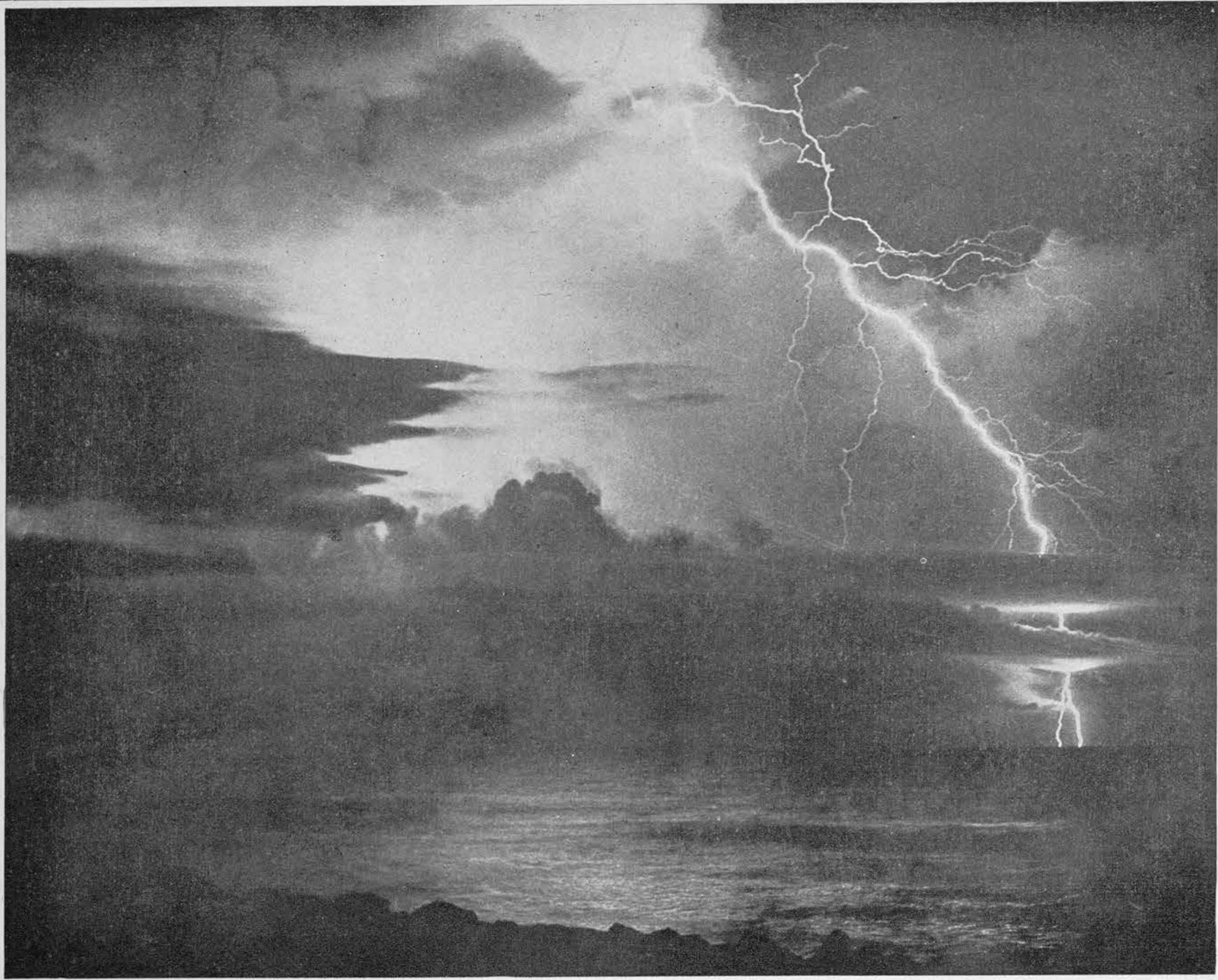
REMARKABLE PHOTOGRAPH OF A LIGHTNING FLASH TAKEN AT MIDNIGHT ON THE ISLAND OF CEYLON. (Photo by Underwood & Underwood.)
