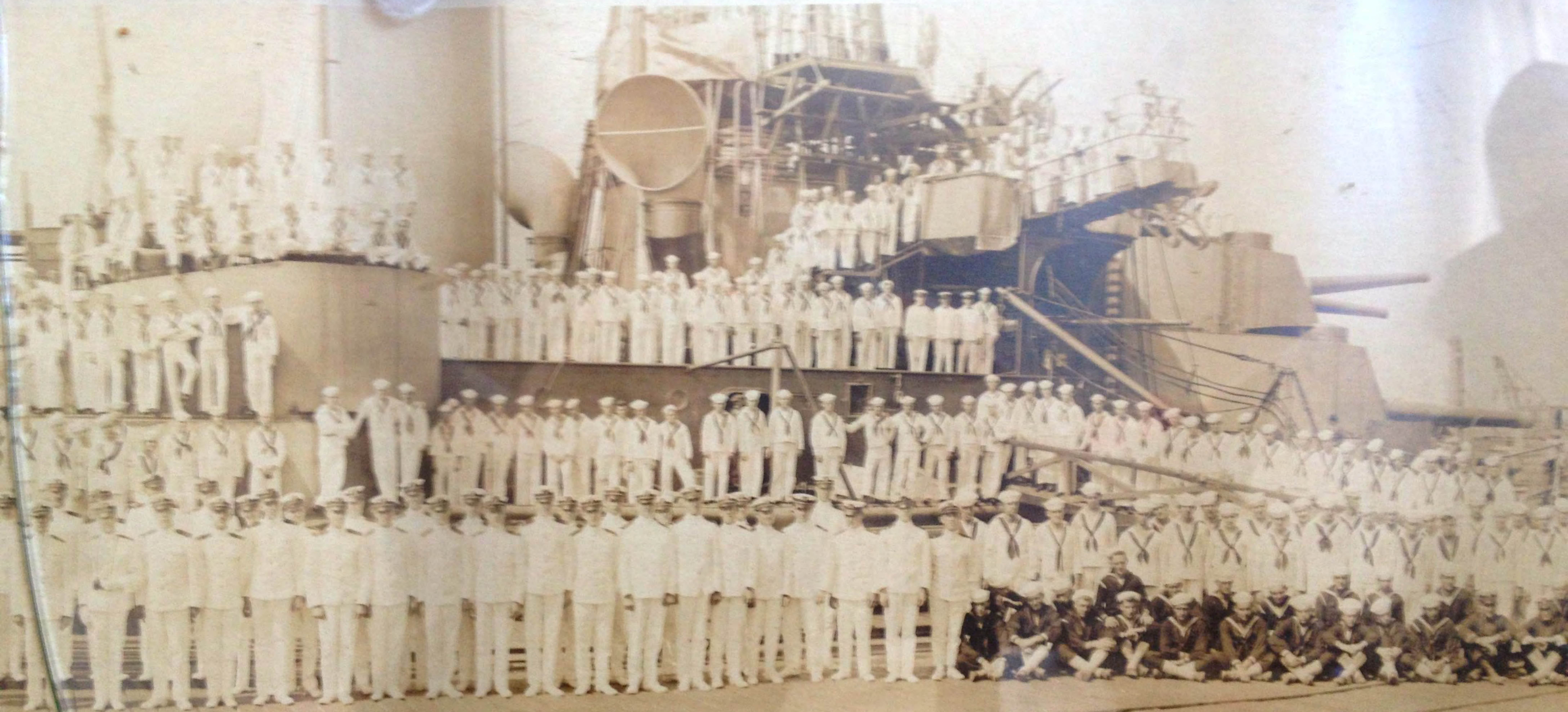
U.S.S. Georgia
