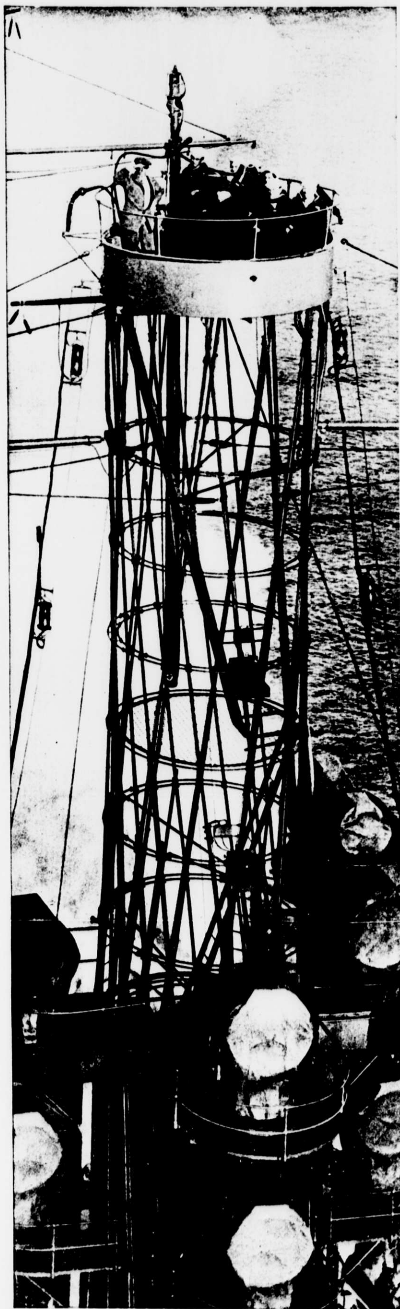
Fire Control Mast. A Distinctive Feature of the New American Warships.
